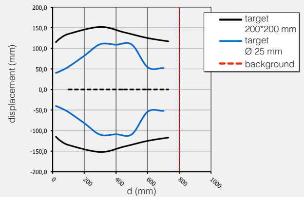
UKR1F/**-** parallel displacement
