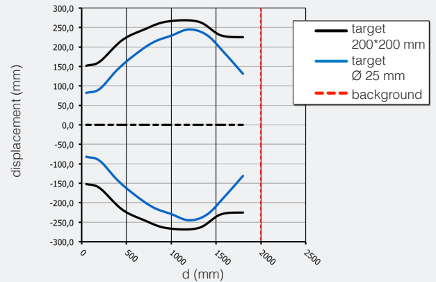
UKR1F/**-** parallel displacement
