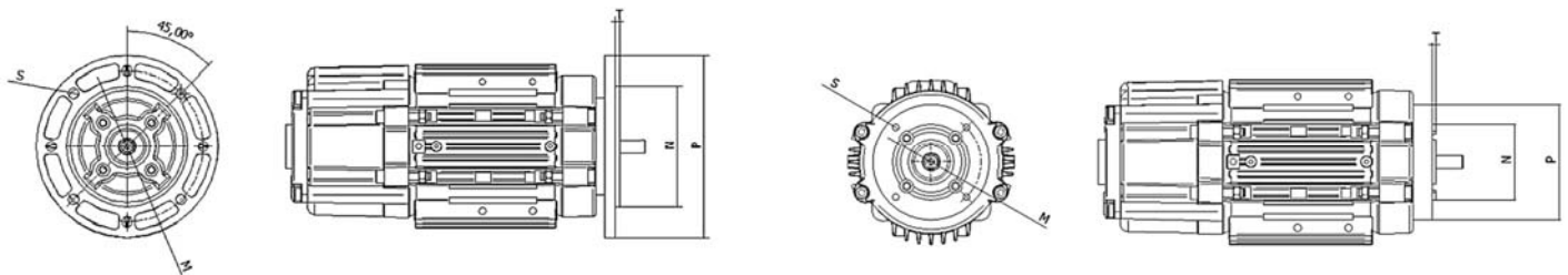
Mounting B3
