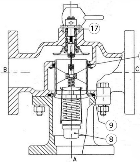
1 1/2" & 2" BM
