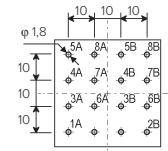
Hole layout (from solder side)
