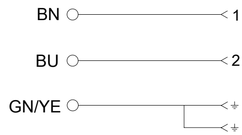
ELECTRICAL DIAGRAM 00
