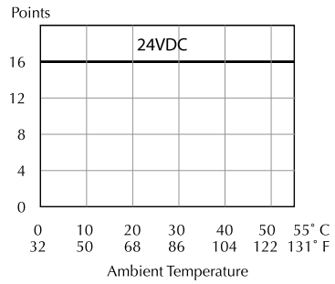
Derating chart
