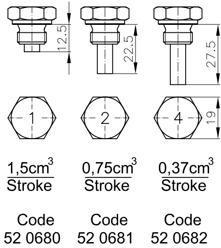
METERING SCREW (EXCHANGEABLE PLUG)
