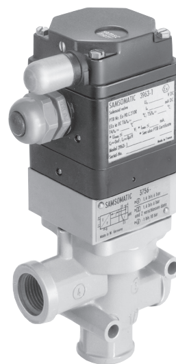
Fig. 2: 3/2-way solenoid valve · Actuated on one side · With spring return mechanism · K_{VS} 4.3 · G \frac{1}{2} connection
