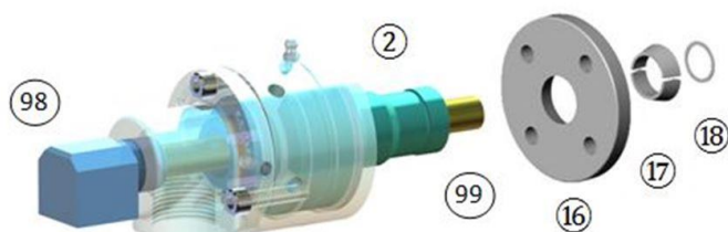
Double Flow
