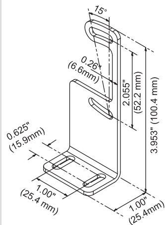
SEB-4 Mounting Bracket With Hardware
