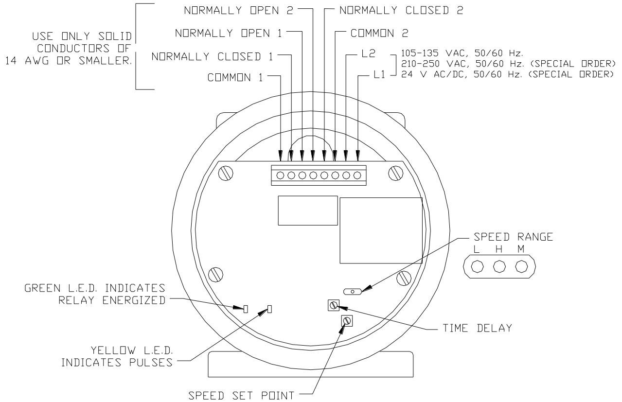
FIGURE 4: Electronics View
