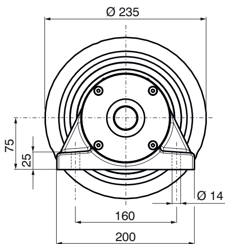
STW 40-50 chuck with shaft end
