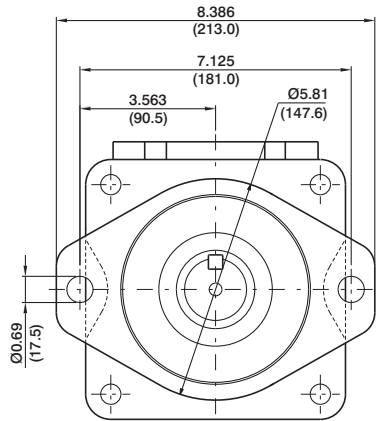
Shaft code 4 SAE CC splined shaft Class 1-J498b 12/24 dp, 17 teeth 30° pressure angle flat root side fit
