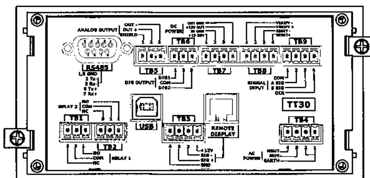
REAR VIEW TACHTROL 30
