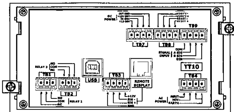
REAR VIEW TACHTROL 10
