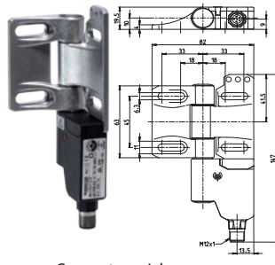
Connector axial Installation position on the right side
