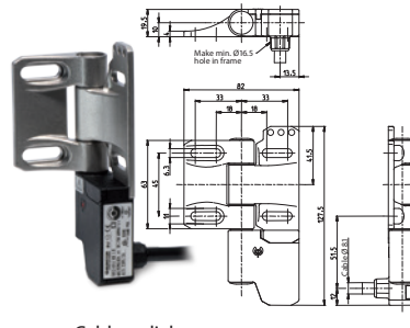
Cable radial Installation position on the right side
