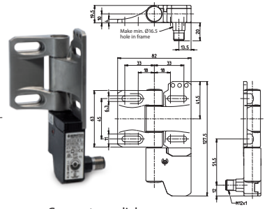
Connector radial Installation position on the right side
