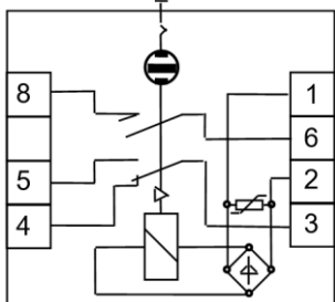
Version with 1 changeover contact and 1 passing contact
