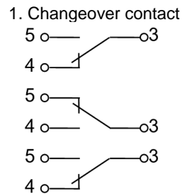
Version with 1 changeover contact operated directly and 1 make contact (NO) in middle position
