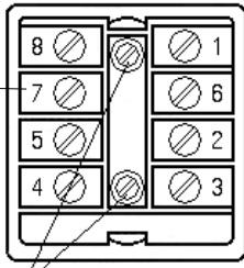
Relay with single coil
