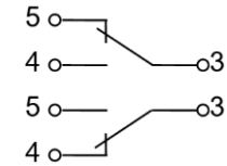
Version with 1 changeover contact operated directly and 1 changeover contact
