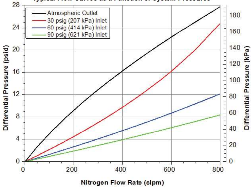
Mott DEF515H Flow Rate vs. Differential Pressure Typical Flow Curves as a Function of System Pressures
