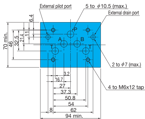
ESD-G03 Mounting Gasket Surface Dimensions Gasket Surface Mounting Dimensions (ISO4401-05-0-05)
