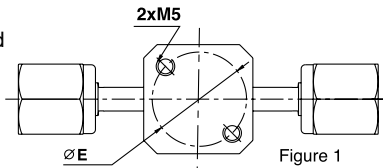
Figure 1 The M5 threaded mounting holes will accept 10-32 screws.
